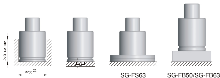
Sposoby mocowania • Assembly possibilities
