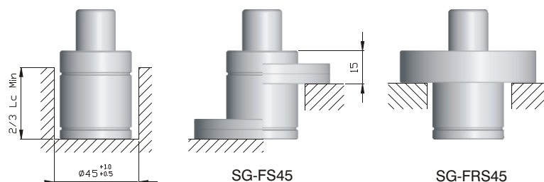
Sposoby mocowania • Assembly possibilities
