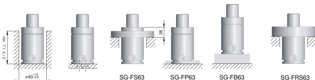
Sposoby mocowania • Assembly possibilities
