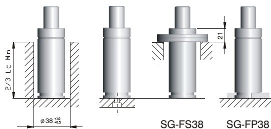
Sposoby mocowania • Assembly possibilities
