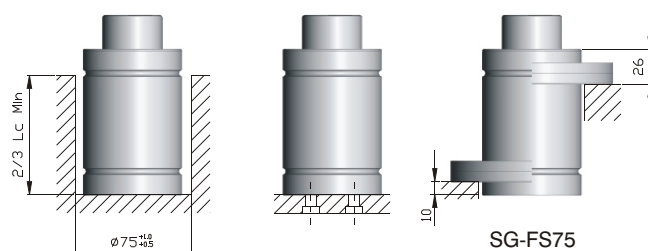
Sposoby mocowania • Assembly possibilities
