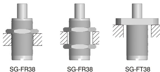
Sposoby mocowania • Assembly possibilities
